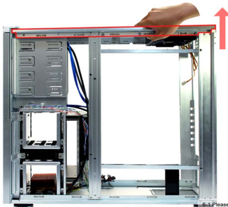
6-1. Please lift the top cover of TJ10
